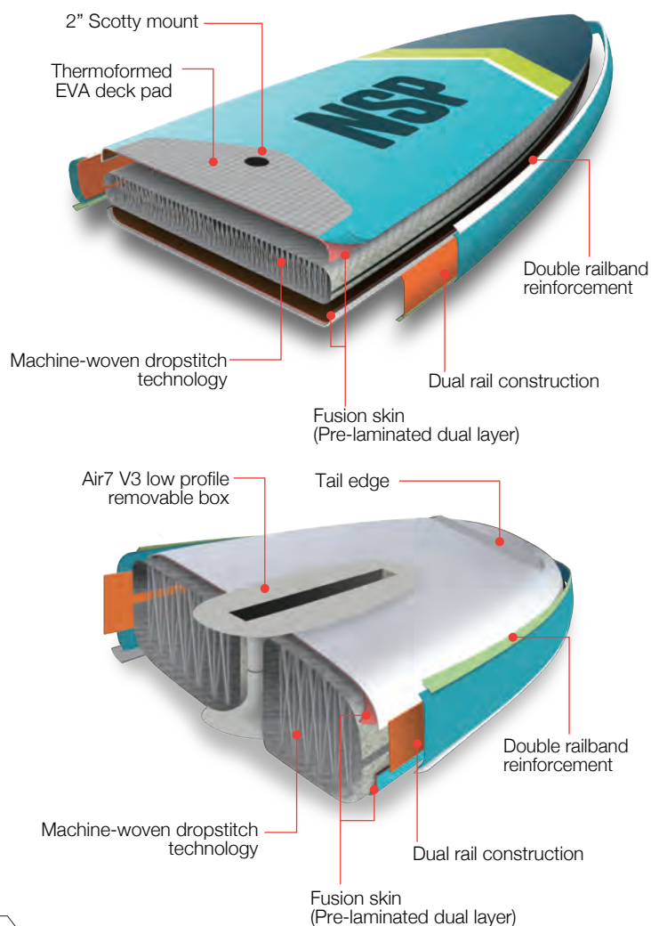
Fusion-reinforced double layer glueless pre-lamination
